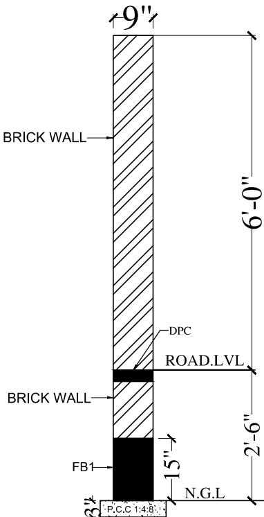
9" TH. BRICK WALL FOUNDATION. (SECTION AT 'A-A')
